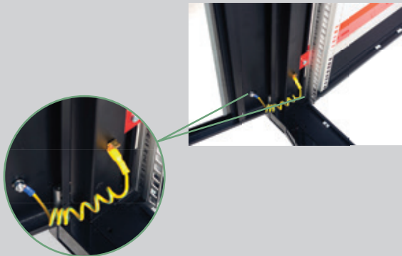
Quick Fix Grounding Terminal Fitted On Frame
